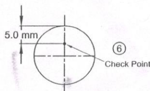
Check Point For Core Hardness On Dia Ø49.8
