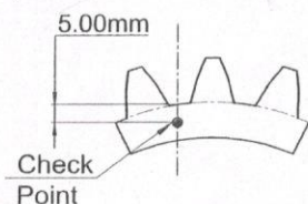
Check Point For Core Hardness On Spline A &amp; B (Ø63) (Ø48)
